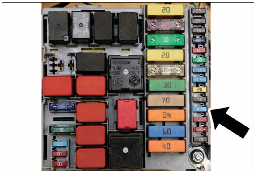
F15 Fuse 15 Amp Blue Cigarette Lighter/Power Outlet Front Console
