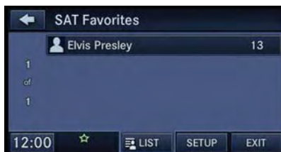
SAT Favorites
