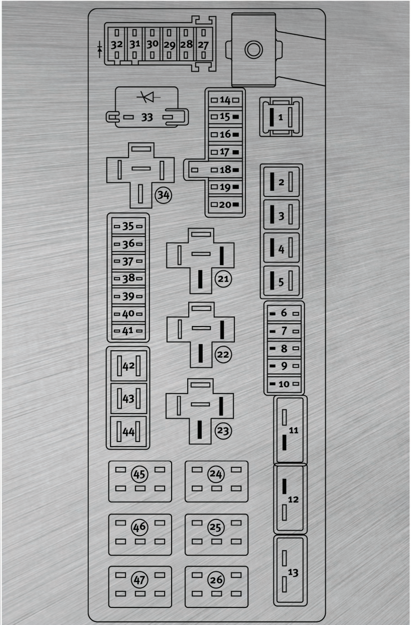
Fuses – Rear Power Distribution Center
