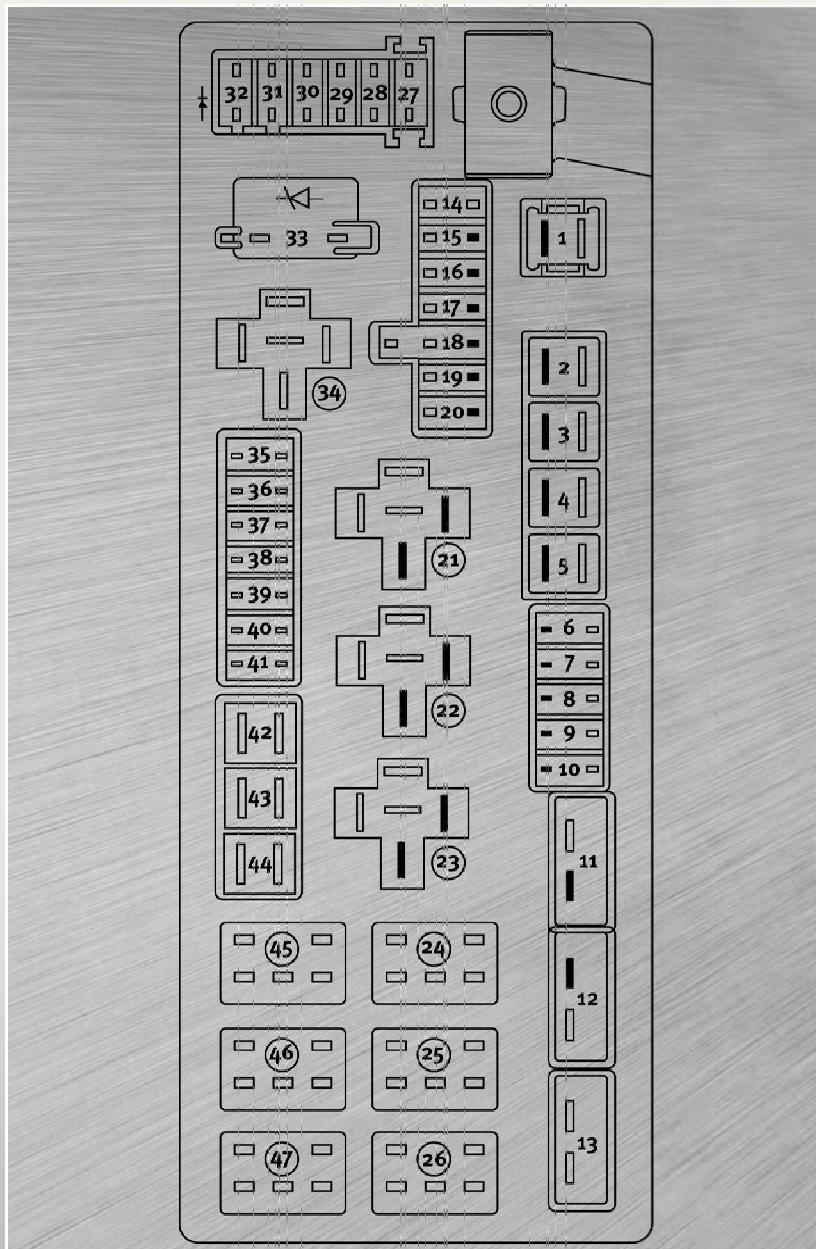
Fuses – Rear Power Distribution Center
