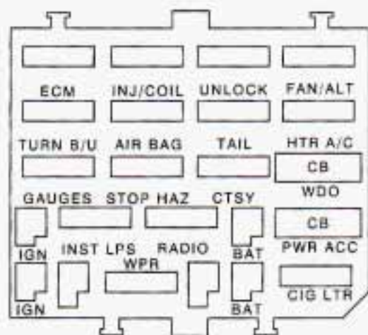
FRONT VIEW OF FUSE BLOCK
