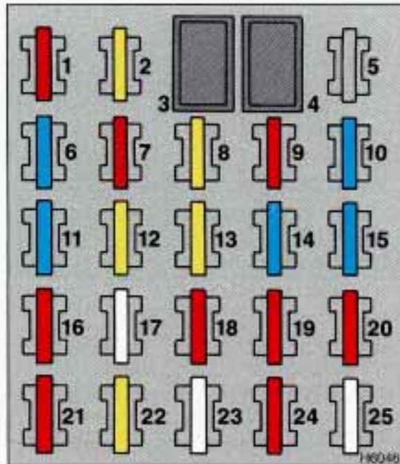
Left Side Fuse Panel
